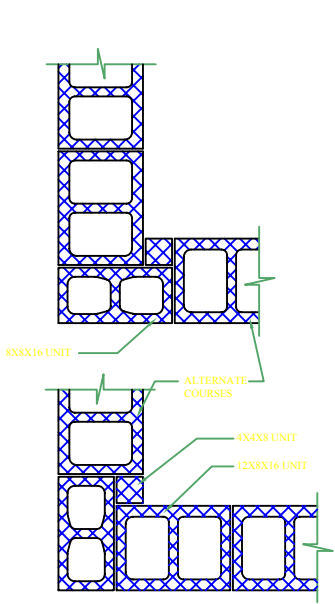
12" WALL CORNER DETAIL
